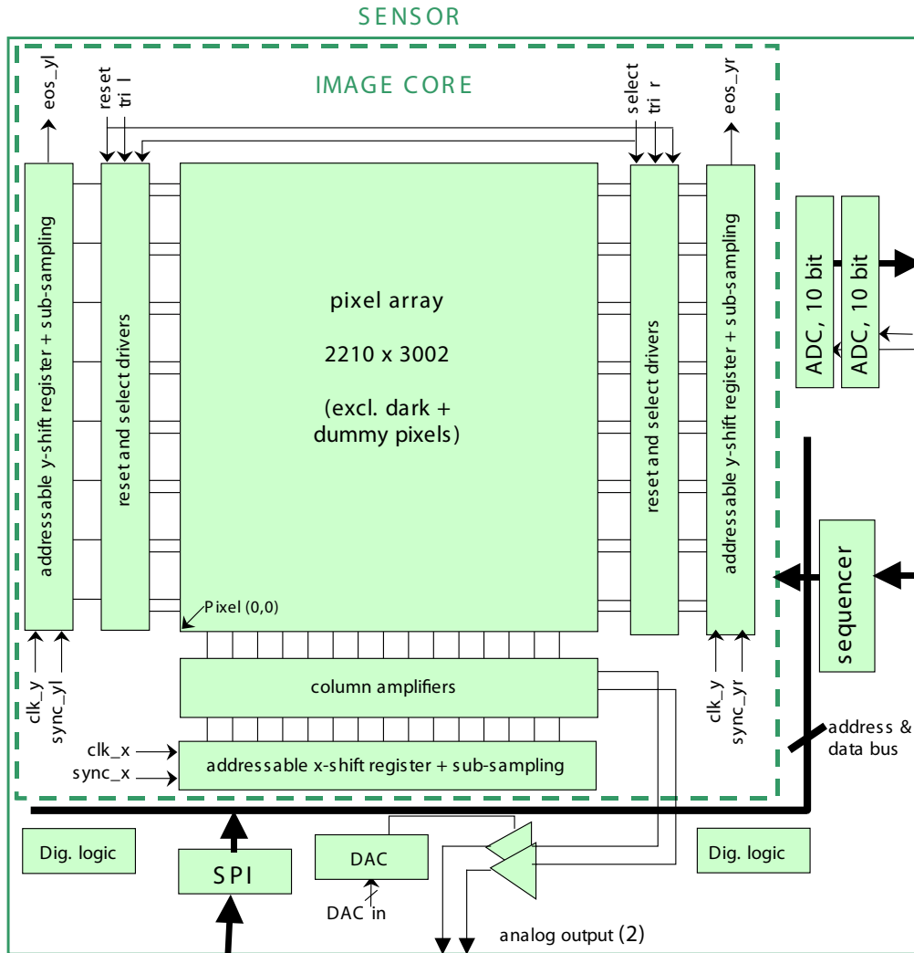
Figure 3. Floor Plan
