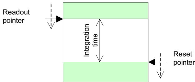
Figure 14. Electronic Rolling Shutter Operation
